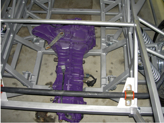
Eagle Medallion transaxle to be used
