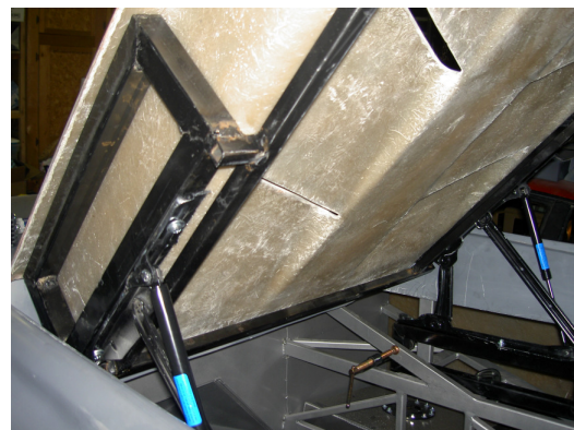
Fabricating engine hatch mounting. Rear wing is mounted
